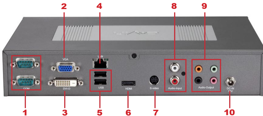
1. RS-232 x 2 2. VGA 3. DVI 4. Ethernet LAN 5. USB x 2 6. HDMI 7. S-Video in 8. Audio-in 9. Audio-Out 10. Power Connector
